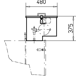
② Schutzgehäuse Protective housing Caisson de protection
